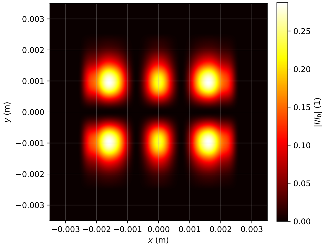
Intensity profile I(x, y, z = 3.503)/I_0 , P_{in}=1.0P_{cr} , artificial time
